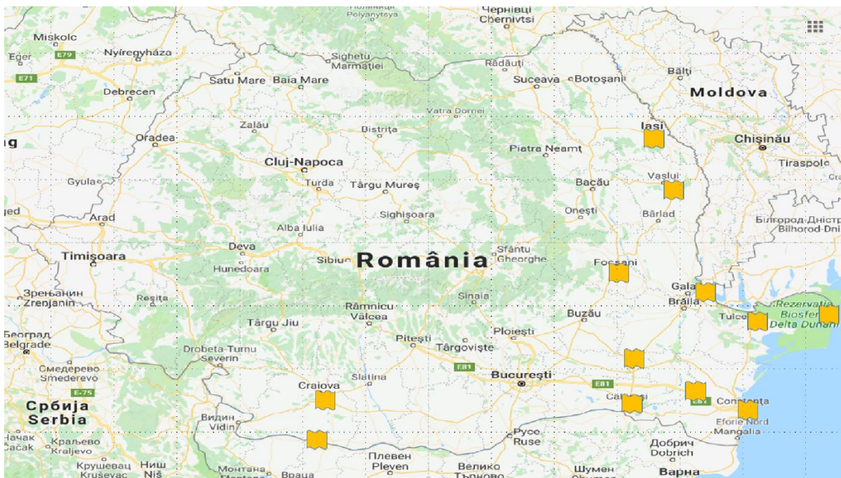
Fig. 1. - Locatiile in care RNSRM a detectat Ru-106 in data de 29.09.2017, prin gamma spectrometrie
