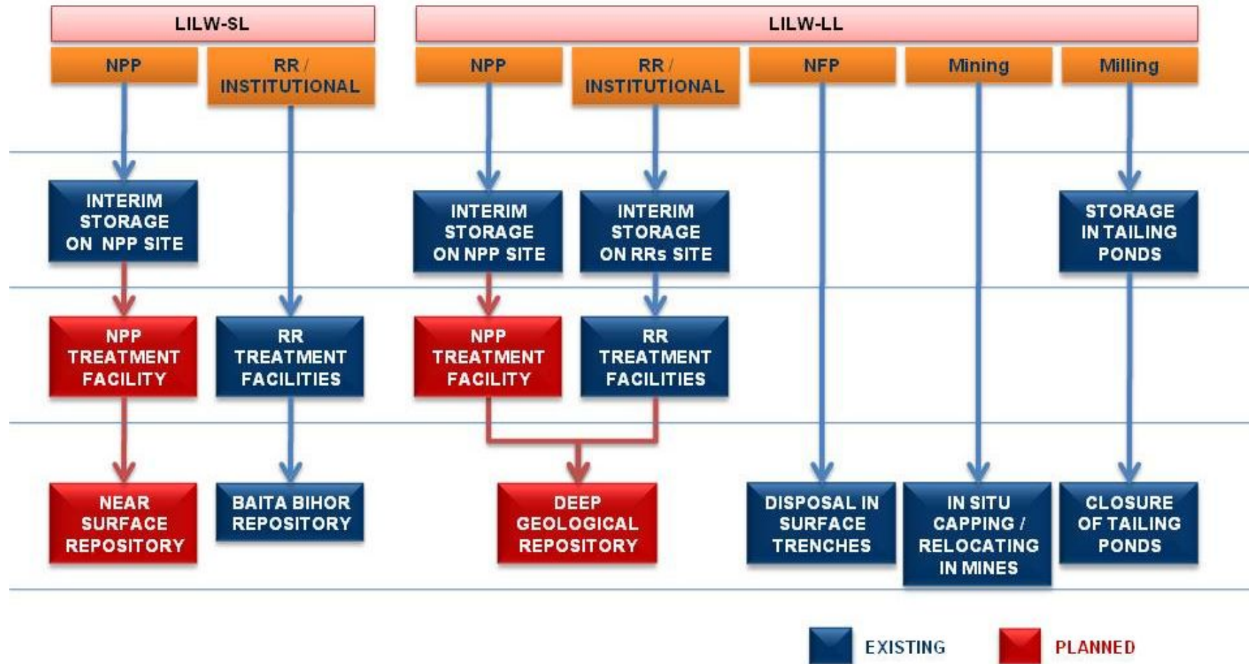
Figure B2: The strategy for the management of RW resulted from operation and decommissioning of NPP and research reactors, institutional activities, nuclear fuel fabrication, uranium mining and milling
